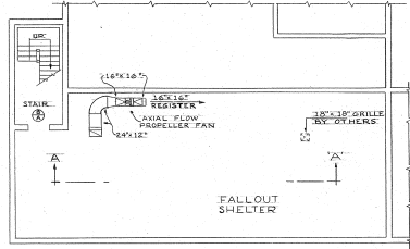
PART FOUNDATION PLAN SCALE 3/8"=1'-0"
