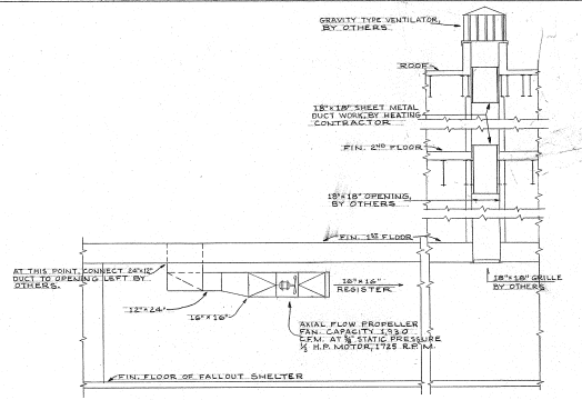
ELEVATION 'A-A' SCALE 3/8"=1'-0"
